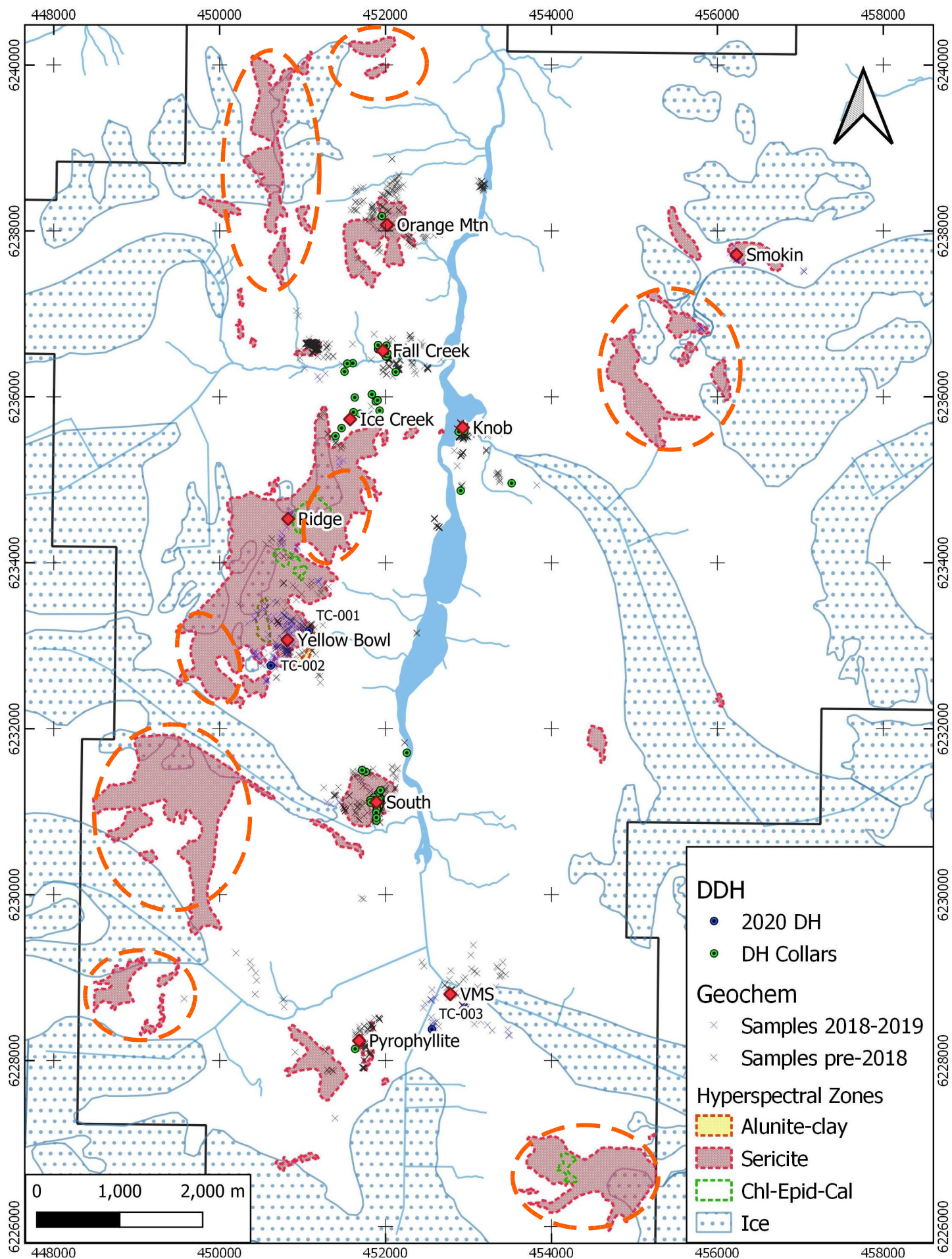
Figure 1: Todd Creek alteration zones, rock sample locations, drill collars, mineralized zones. Red dashed ellipses highlight unexplored and unsampled alteration zones.
